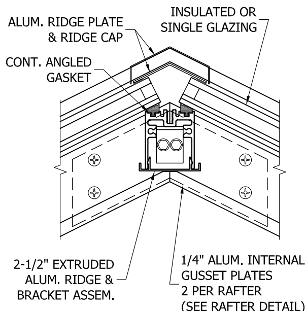
RIDGE D
