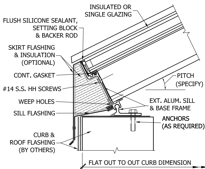
CURB/SILL A
