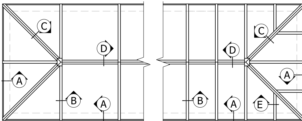
HIP-RIDGE PLAN VIEW
