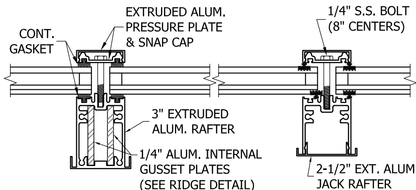
B RAFTER
