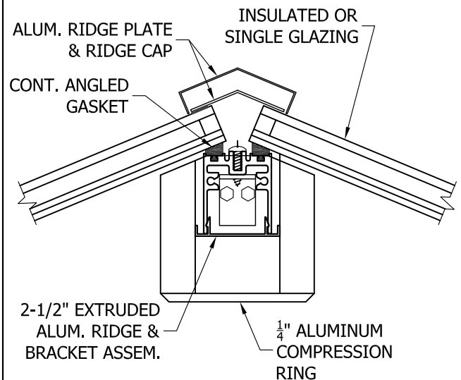
RIDGE D
