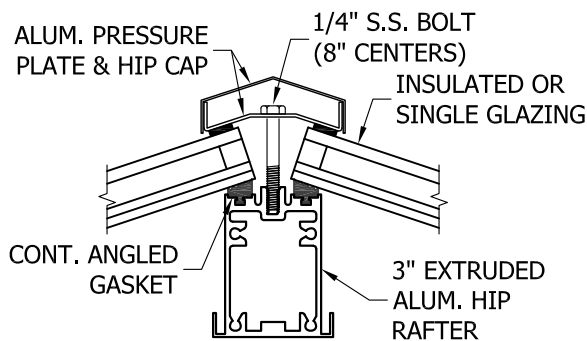
HIP C
