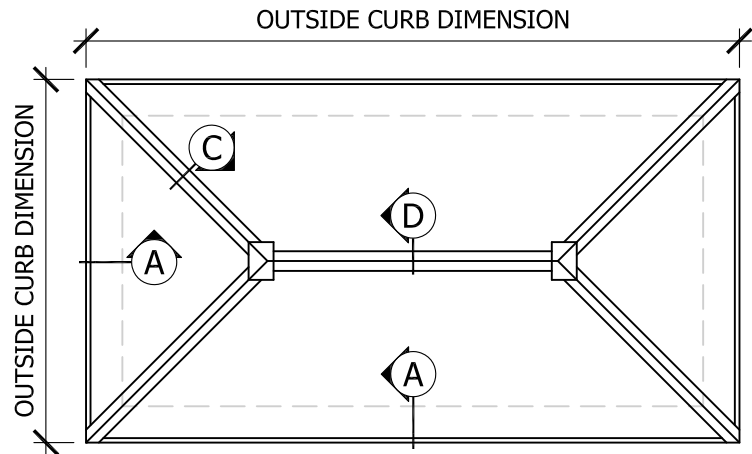
HIP-RIDGE PLAN VIEW
