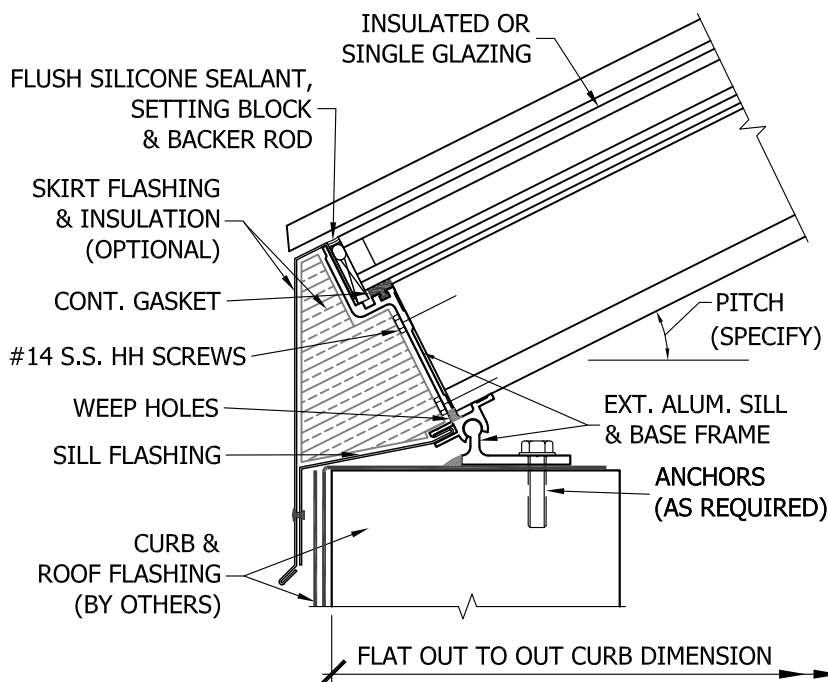
CURB/SILL A
