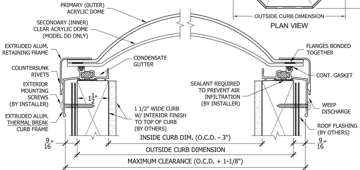
ELEVATION VIEW
