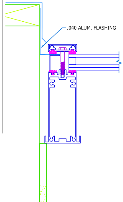
(A) END WALL DETAIL
