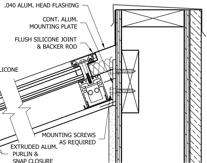
HEAD DETAIL B
