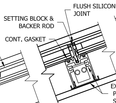
PURLIN DETAIL E (IF APPLICABLE)
