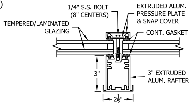
3" RAFTER C
