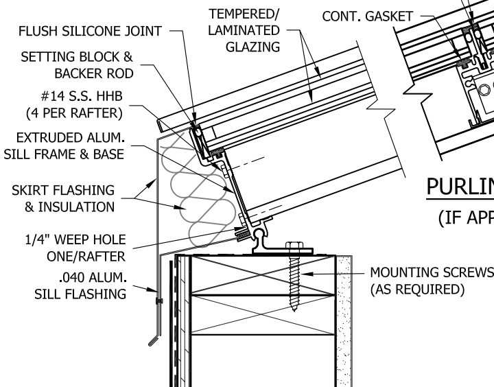
SILL DETAIL A
