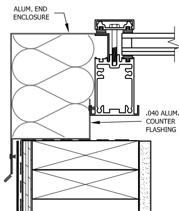
RAFTER/CURB D
