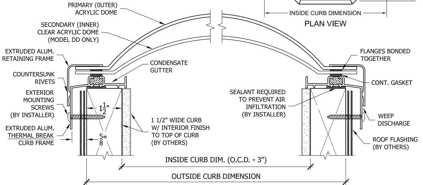
ELEVATION VIEW
