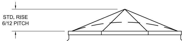
ELEVATION VIEW
