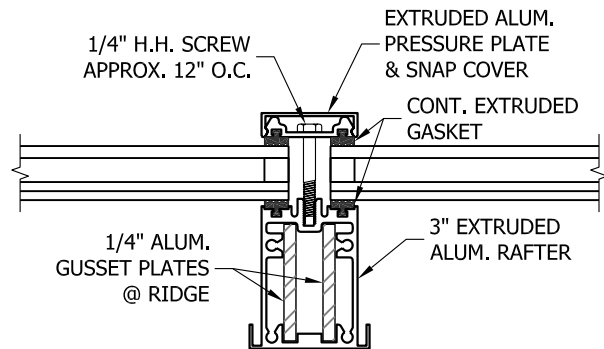
C RAFTER DETAIL QUATER SCALE
