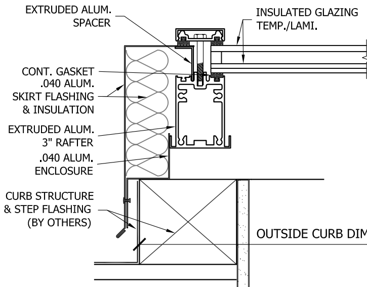
B CURB/SILL DETAIL QUATER SCALE
