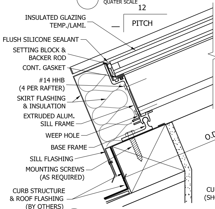
A CURB/SILL DETAIL QUATER SCALE
