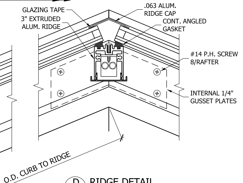
D RIDGE DETAIL QUATER SCALE
