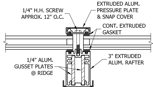
C RAFTER DETAIL
