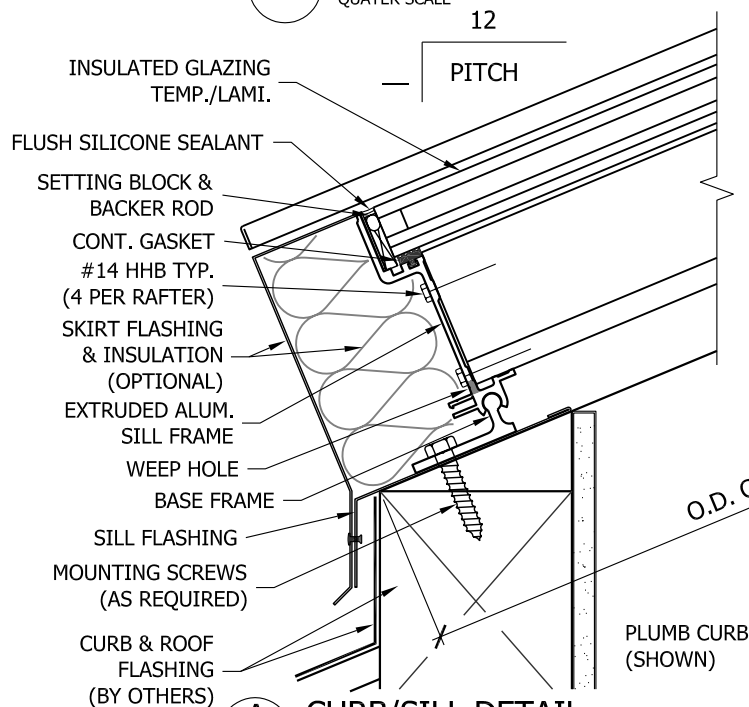
A CURB/SILL DETAIL
