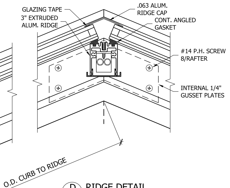
D RIDGE DETAIL
