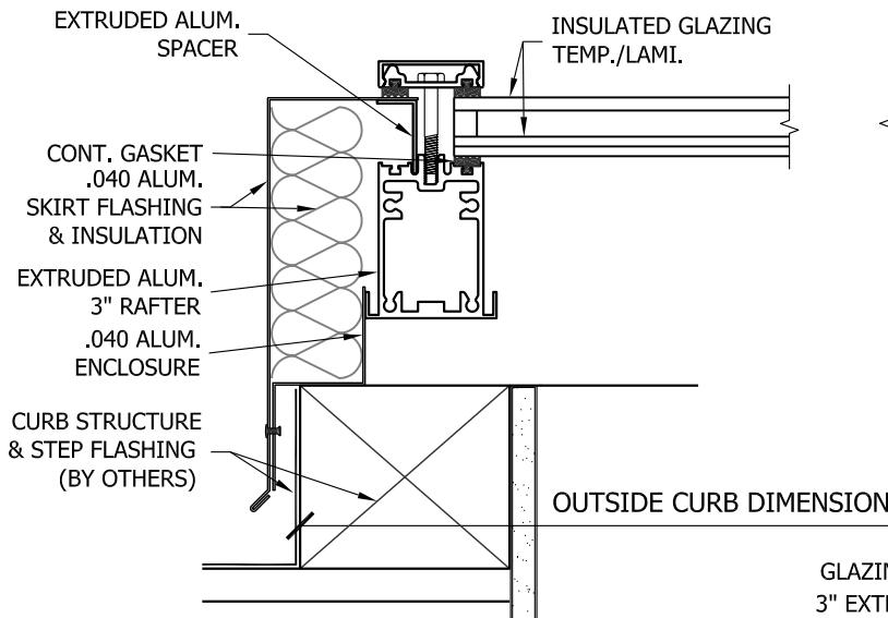
B CURB/SILL DETAIL
