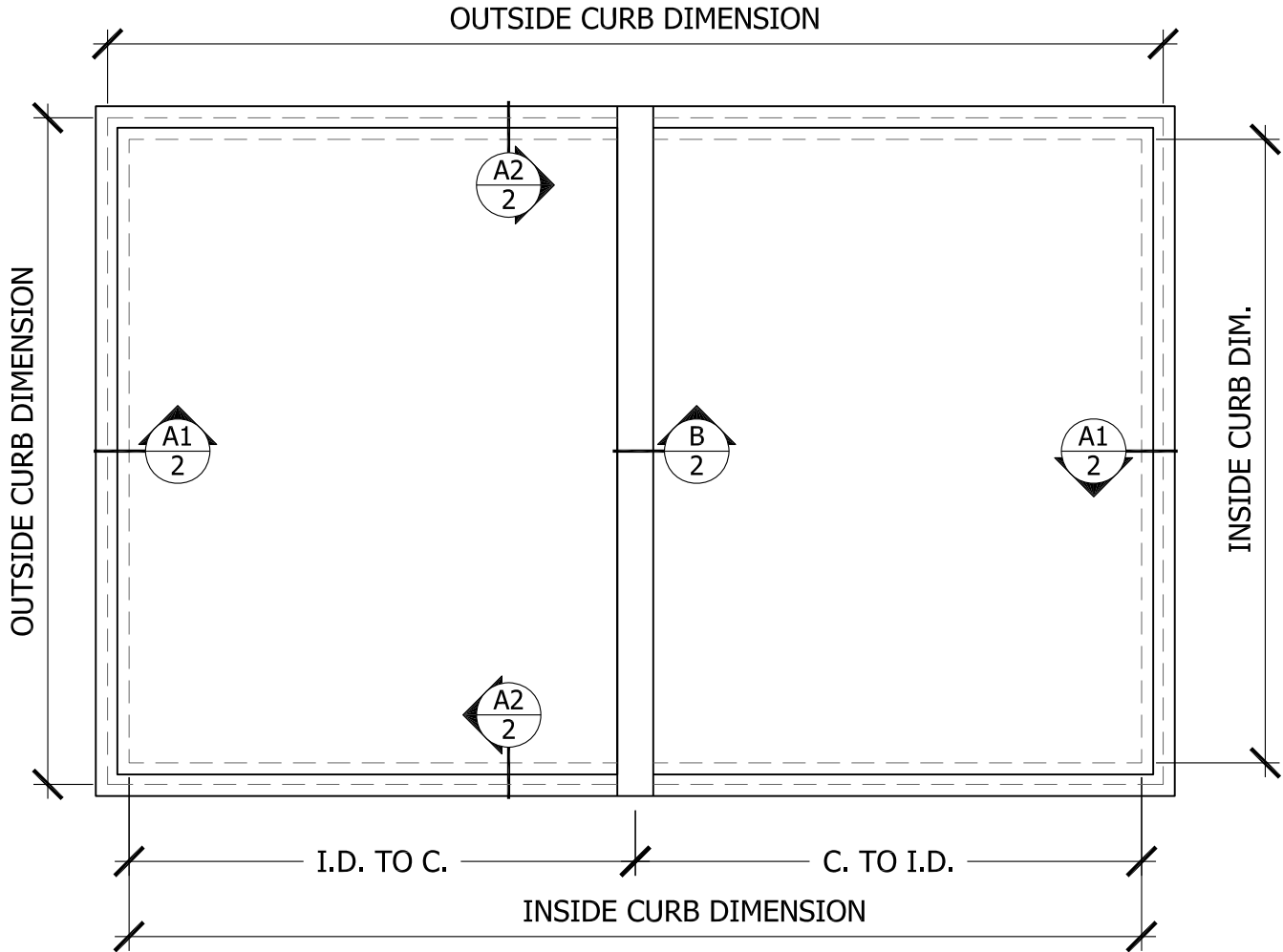
PLAN VIEW (TRUE VIEW)
