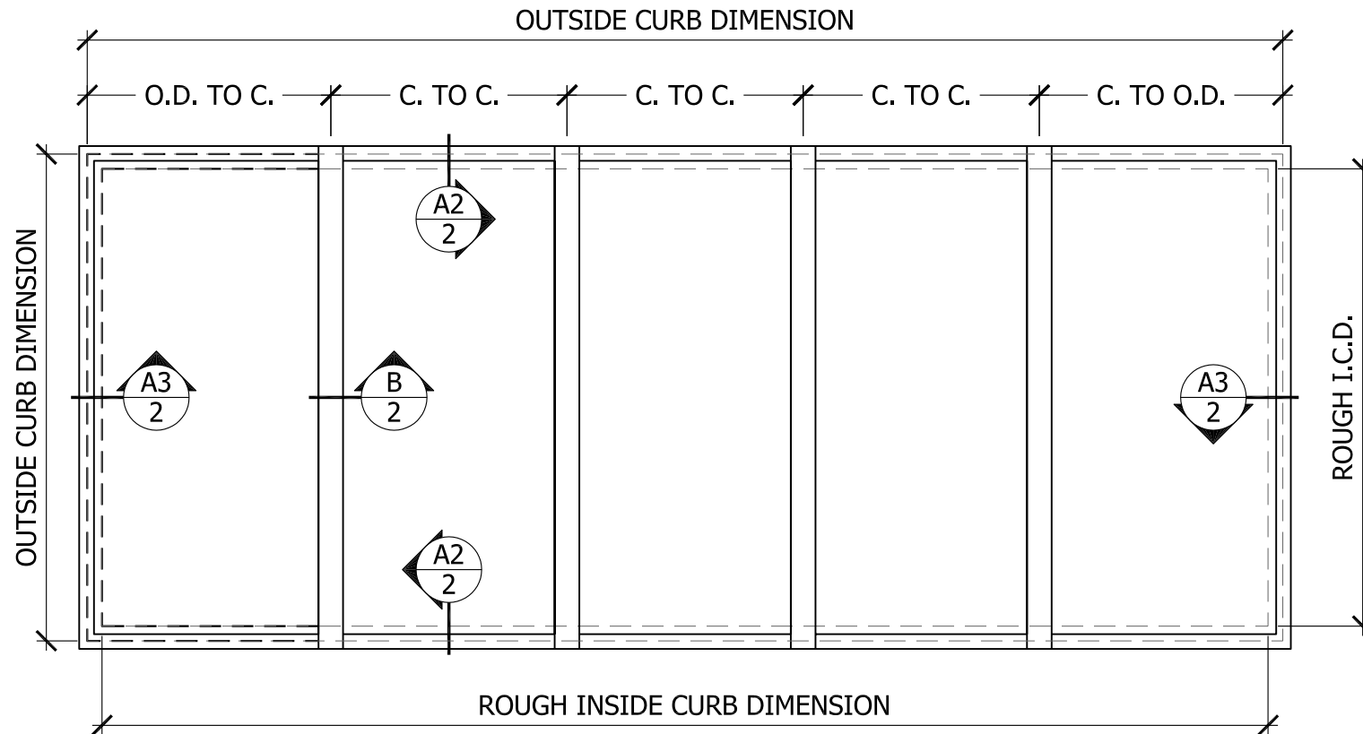
PLAN VIEW (TRUE VIEW)
